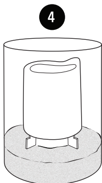
Cover Diameter: 3.4" Height: 4"
